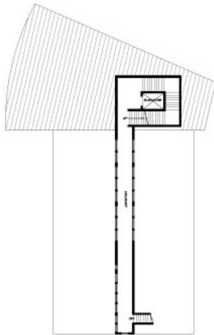
RECREATION WING/ TOWER LEVEL 03
